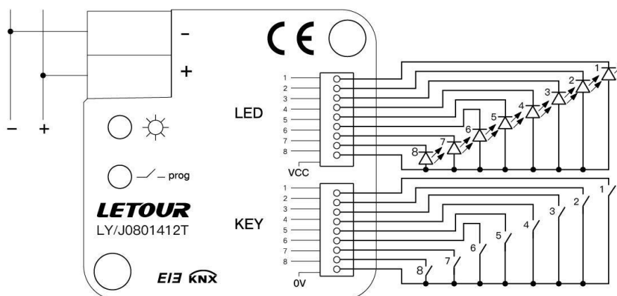
common-anode
