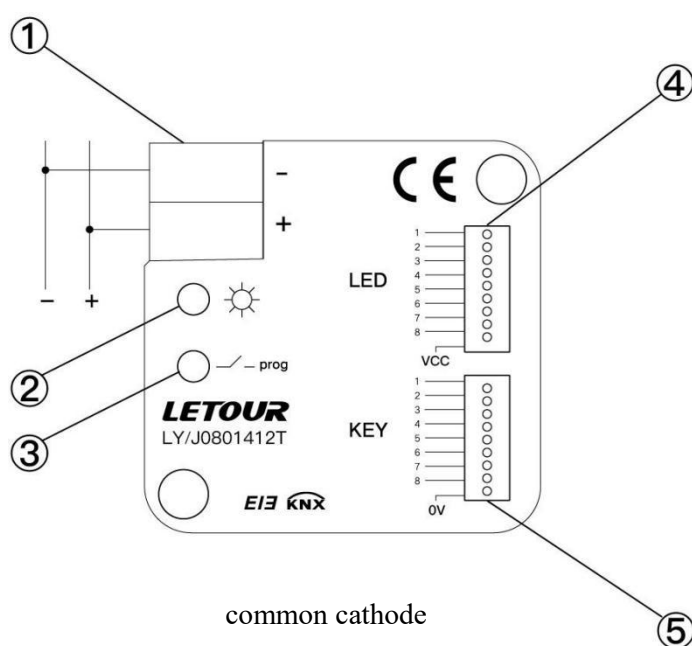
common cathode
